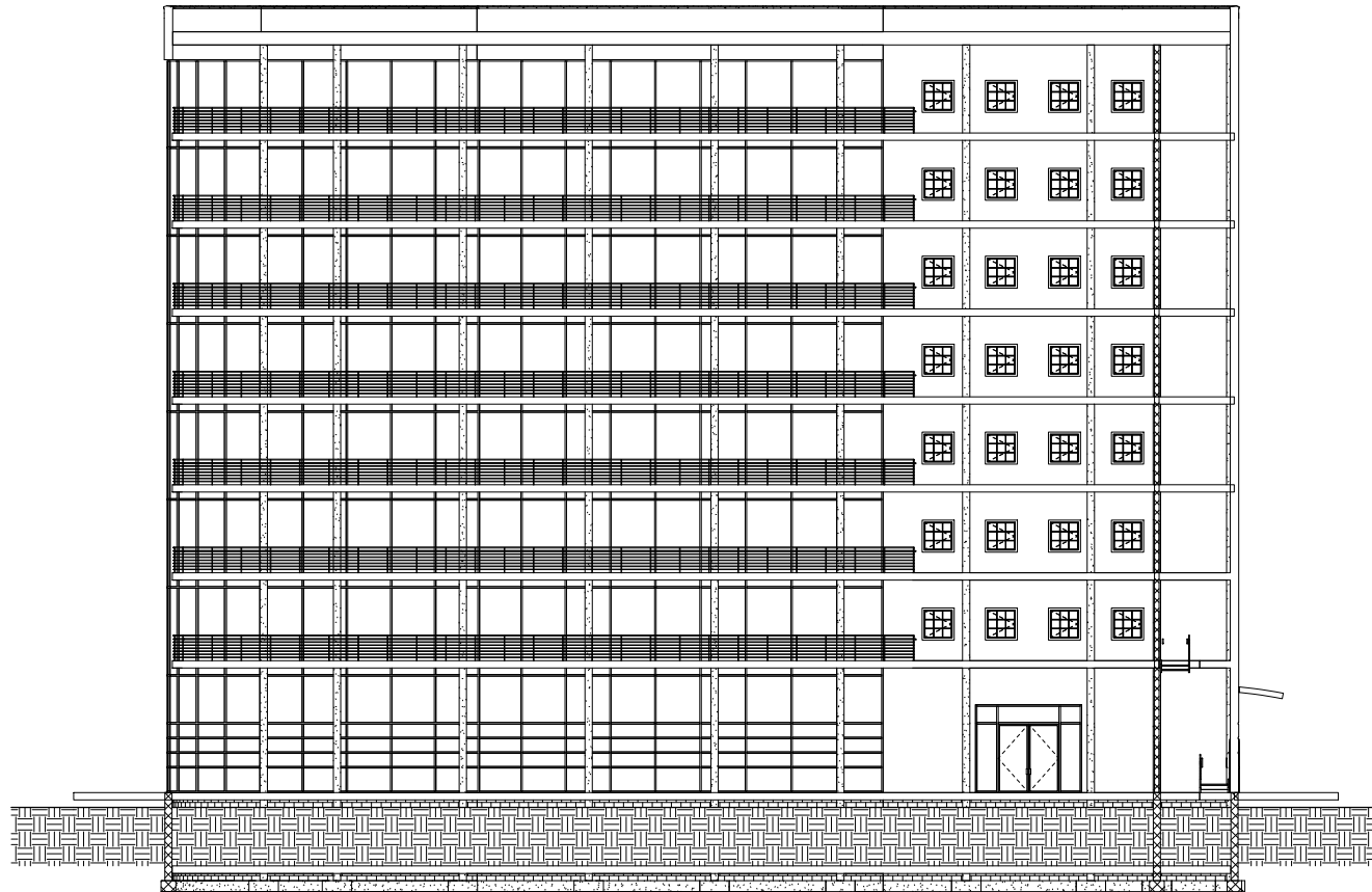
1 East-West Building Section 1/8" = 1'-0"
